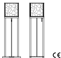
52610 Stand con lampada colore bianco Lamp stand white colour cm 45 x 35 X h 136 in 17 3/4 x 13 3/4 X h 53 1/2
